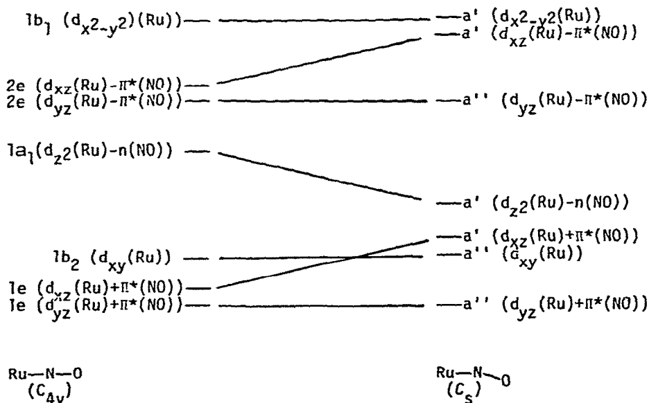
Fig. 1. Energy level diagram for linear and bent {RuNO} complexes. Based on diagrams given in refs. 8, 25 and 31-33.
